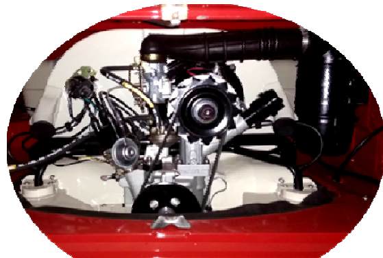
engine: assembled, new parts, cables and tubes
