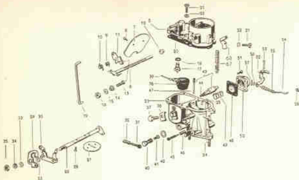
Fig. 18-E — O carburador Solex 30 PIC
